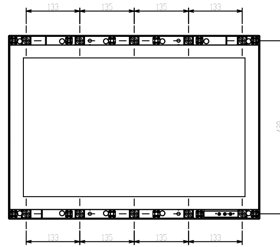
Without design panel Installation screw position
