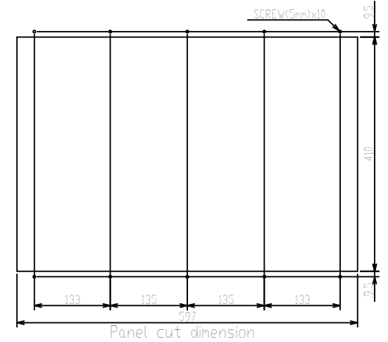
Panel cut dimension
