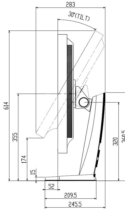
HIGHEST POSITION
