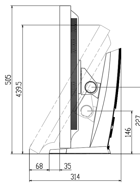
LOWEST POSITION
